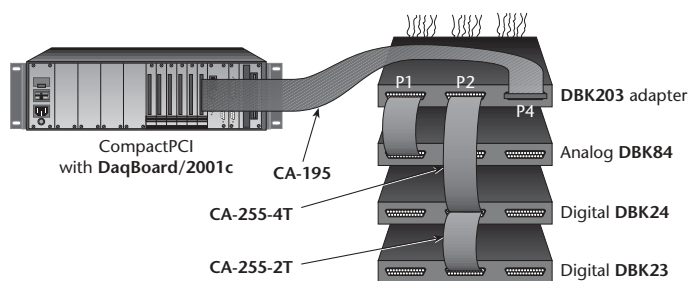
The DBK203 adapter with screw-terminal connectors
