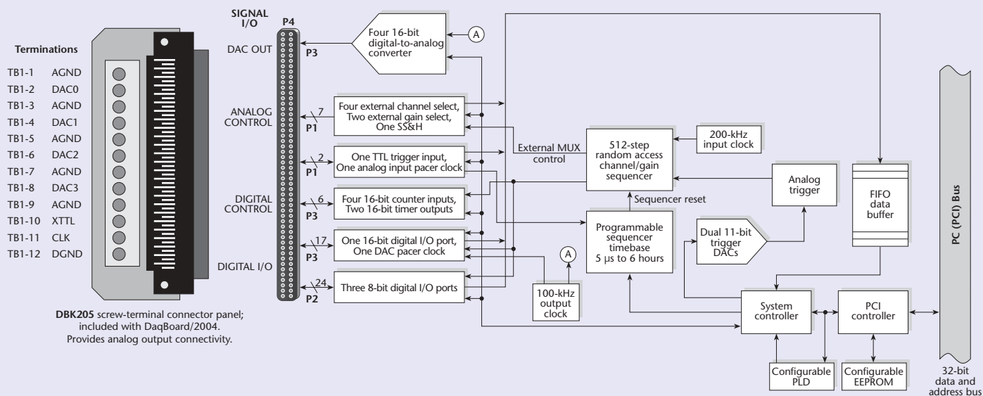
DaqBoard/2004 Block Diagram
